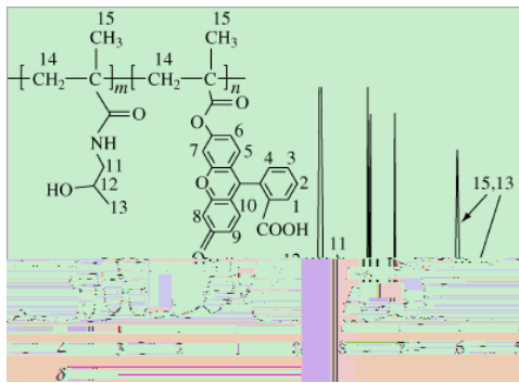
P(HPMA-FMA)
